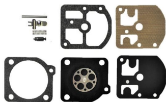
707787 KIT REPARO CARBURADOR 43/52CC
